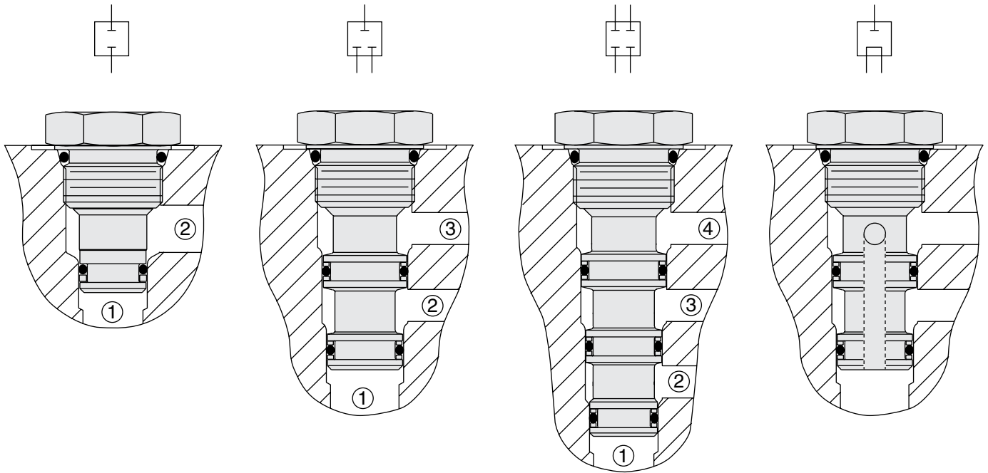
2-Way Cavity CPXX-20-X
